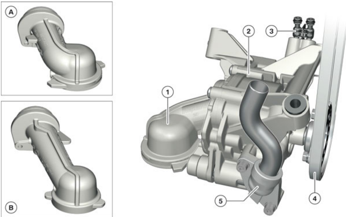
N63TU2 engine, oil intake snorkel
